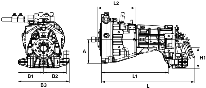
V-Drive Direct Mount
