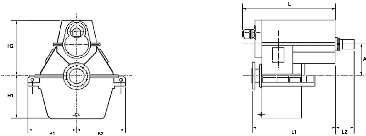
Vertical Offset Remote Mount
